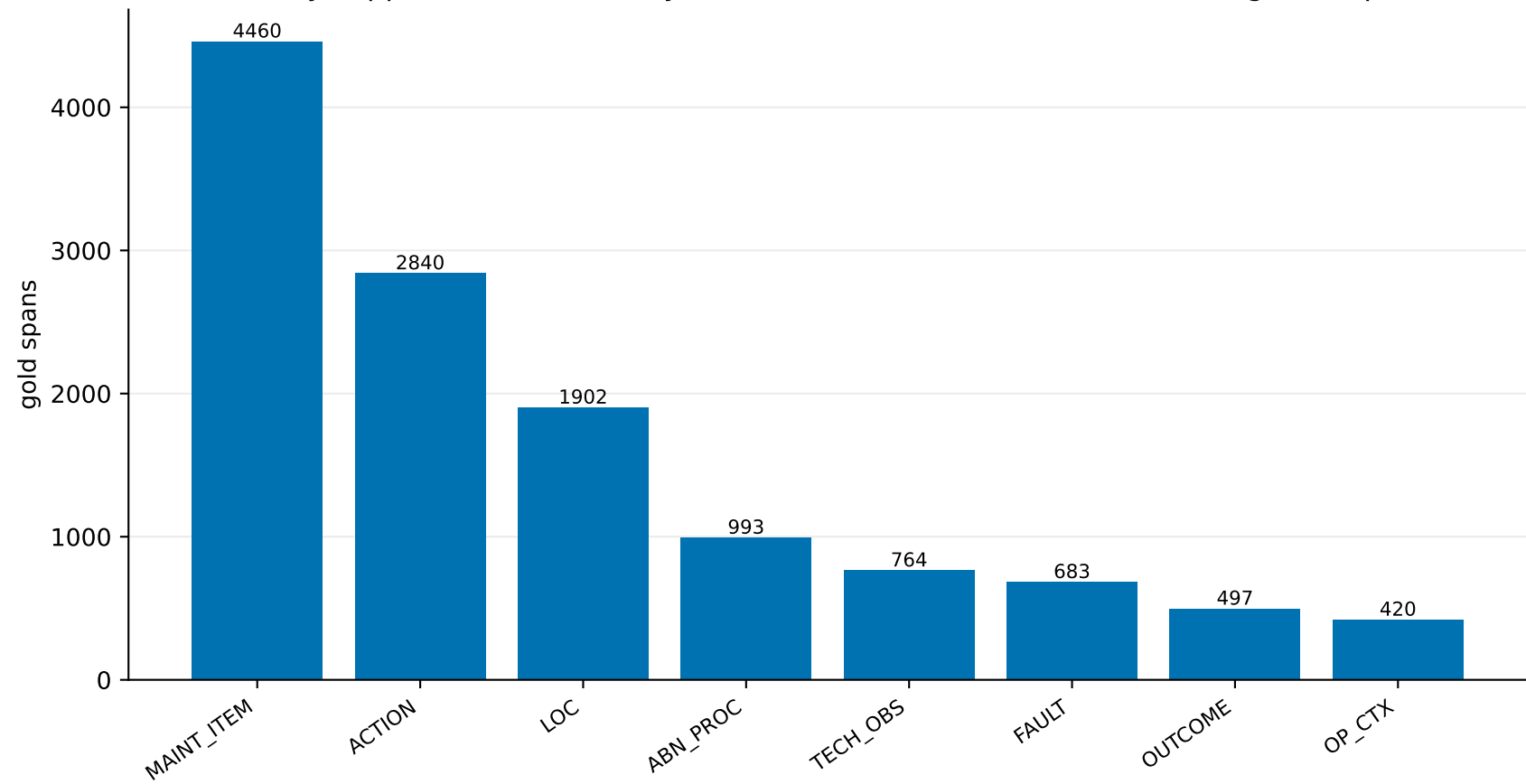
Entity support — Core 8-entity / 10-relation schema full 1,600-record gold corpus
