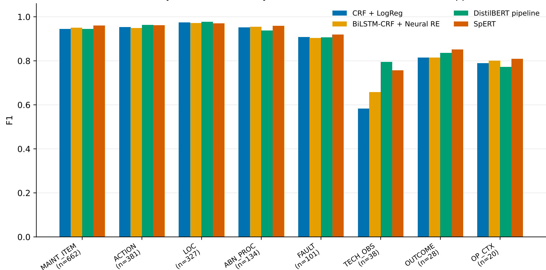
Per-class entity F1 — Core 8-entity / 10-relation schema (frozen TEST support)
