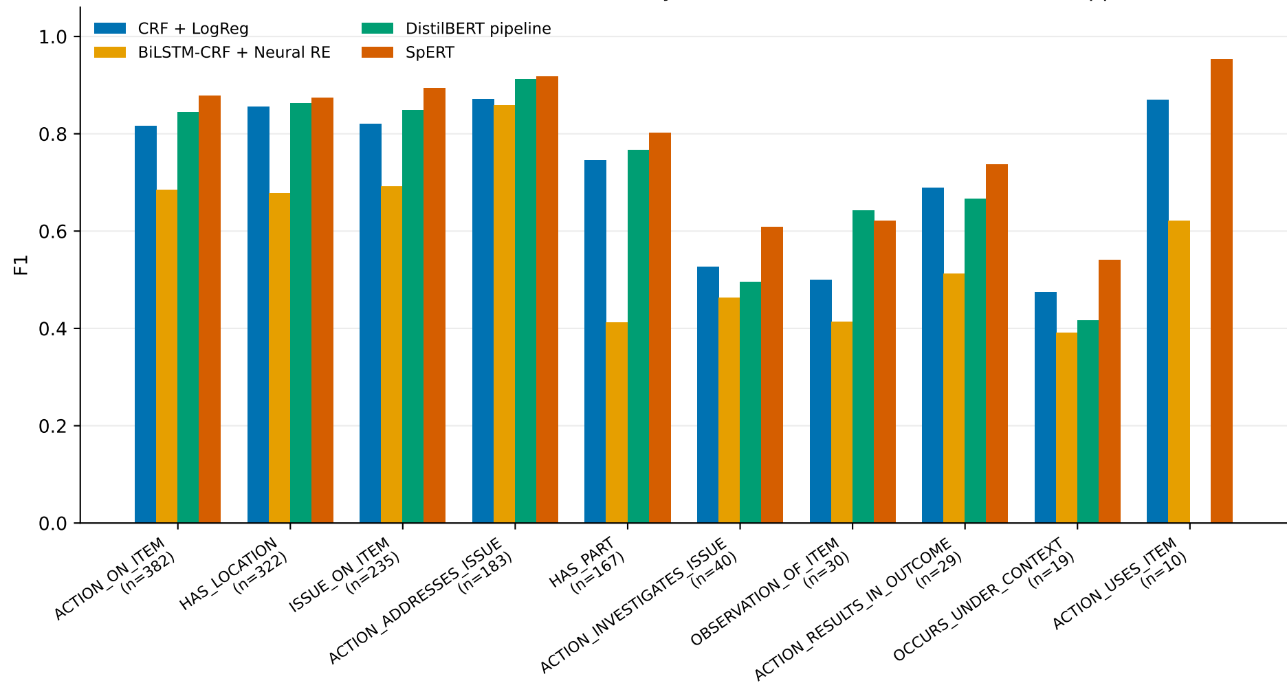
Per-class strict relation F1 — Core 8-entity / 10-relation schema (frozen TEST support)
