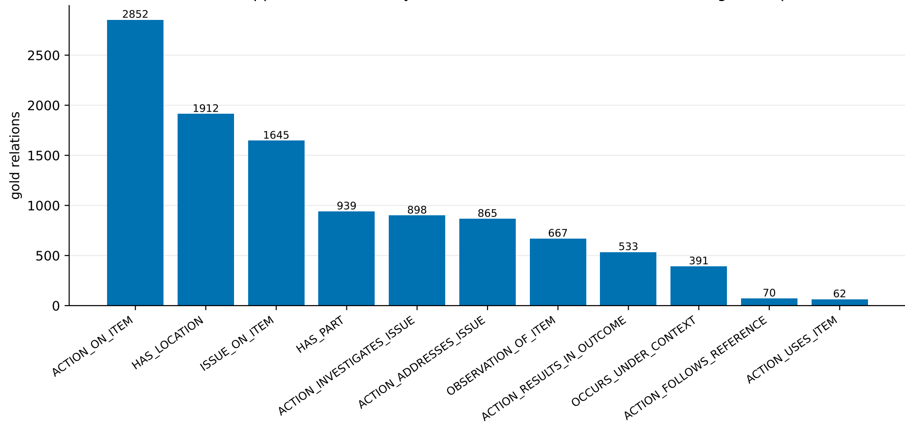
Relation support — Full 9-entity / 11-relation schema full 1,600-record gold corpus
