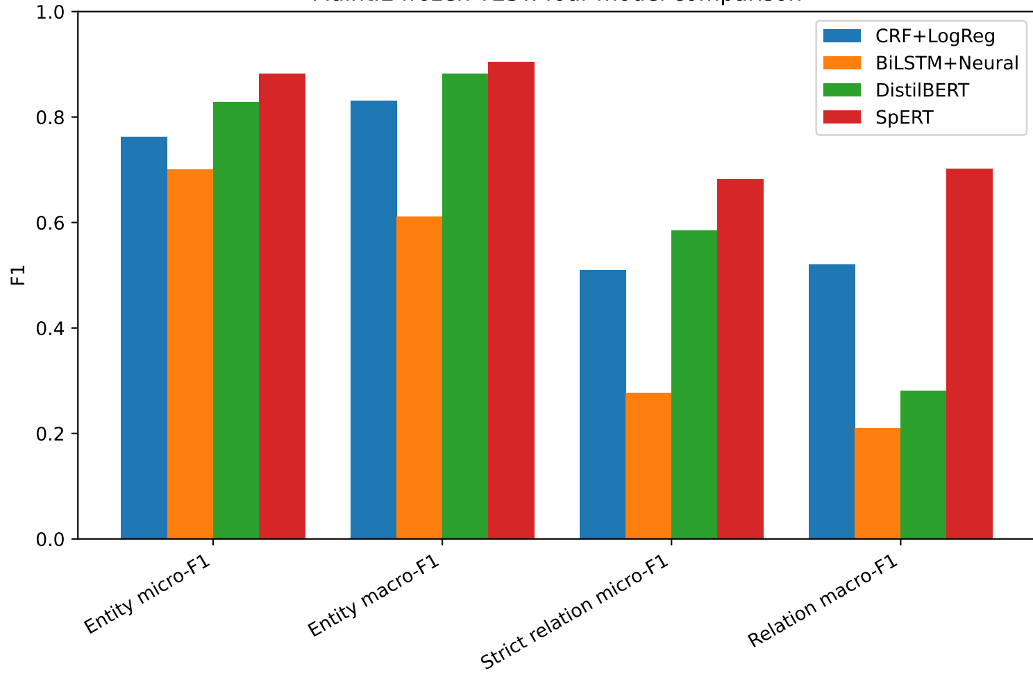
MaintLE frozen TEST: four-model comparison
