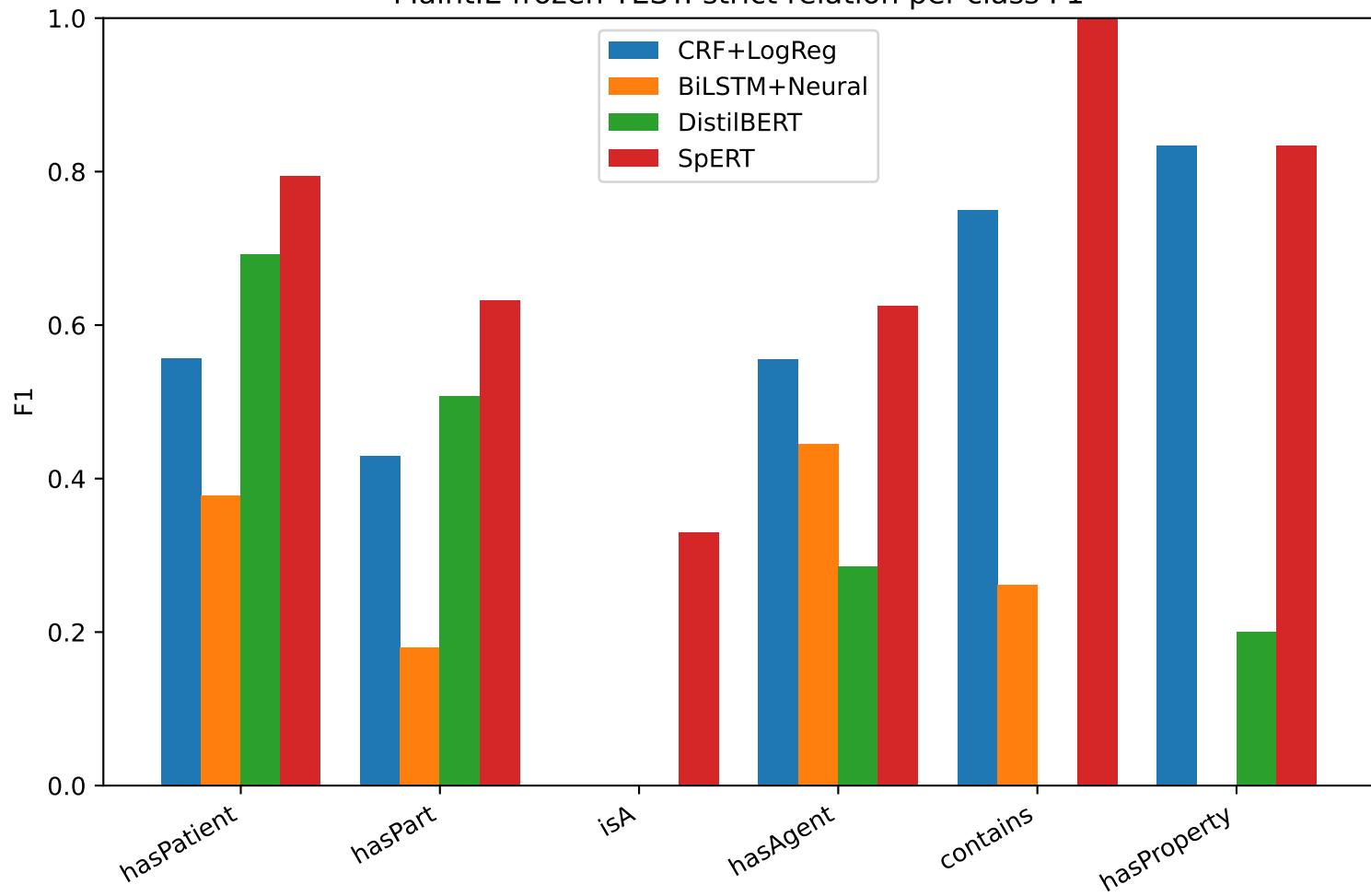
MaintIE frozen TEST: strict relation per-class F1
