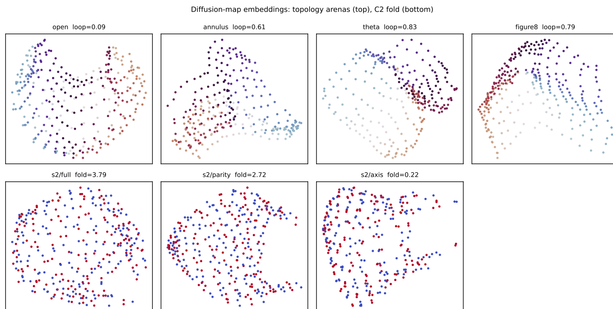
Figure S6. Diffusion-map embeddings. Top: topology arenas, coloured by arena angle. The open arena shows no angular loop in the leading diffusion coordinates (loop score 0.09), whereas the annulus, theta and figure-8 arenas do (0.61–0.83); the manifolds nonetheless remain moderately high-dimensional (intrinsic dimension 5–7), consistent with the persistent-homology result that a single loop is recoverable but higher-genus topology is not. Bottom: the C_2 fold, coloured by orbit tag. The diffusion distance between a position and its 180^\circ image, in units of the distance to a spatial neighbour, is 3.79 under full and 2.72 under parity but collapses to 0.22 under axis : the fold is a property of the diffusion geometry, not of any linear projection.
