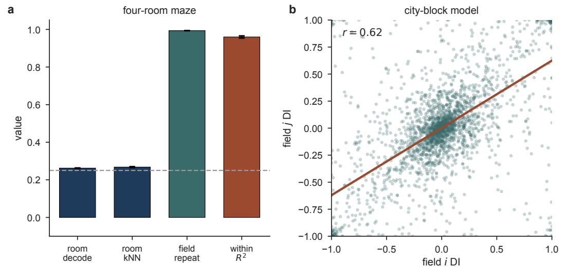
Figure 2. The predictive model reproduces place-field repetition. (a) The four-room maze of Spiers et al. (2015), model ( n = 8 ): four translation-related identical rooms fold onto one map. The room decodes at 0.262 by a generalising decoder and 0.268 by a nearest-neighbour classifier at cells it has already seen, against a chance of 0.25 (dashed): a small residual, but a reliable one ( p = 0.008 ). Fields repeat across the rooms (repetition 0.99) and within-room position stays intact ( R^2 = 0.96 ). (b) A predictive network trained on a city-block maze shows the directional-repetition signature, predicted before any comparison to animal data: the directional index of a field ( i ) against that of its same-orientation partner ( j ) is positively correlated ( r = 0.62 ; scatter subsampled for display, statistic from all pairs). Line, least-squares fit. An exploratory, non-diagnostic reanalysis of real CA1 data testing the same prediction is in the Supplementary Information (Fig. S10).
