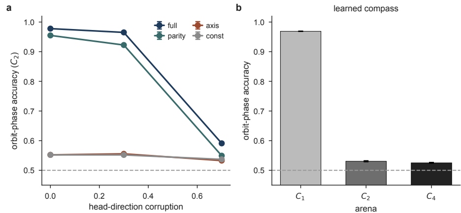
Figure 9. The quotient survives a degraded and a learned compass. (a) Compass corruption during training: orbit-phase accuracy in the C_2 arena for networks that developed with a heading signal randomised on a given fraction of steps (chance 0.5, dashed). The non-invariant encodings ( full , parity ) degrade smoothly, while the invariant ones ( axis , const ) stay pinned at chance. This is a network that grew up with an unreliable compass, and it is not the lesion: an adult lesion is modelled by silencing the compass at test time (Fig. 11), because randomising a compass an adult network already trusts contradicts its egocentric view rather than falling silent, and drives it off its training manifold. (b) A learned, angular-velocity compass, by arena: it resolves C_1 (0.97) but folds C_2 and C_4 to chance, building the quotient with no imposed encoding.
