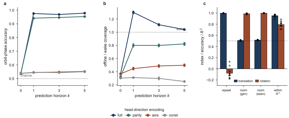
Figure 8. Functional consequences of the fold. (a) Orbit-phase decoding accuracy vs prediction horizon k in the C_2 arena (chance 0.5); the non-invariant encodings ( full , parity ) resolve the fold at k \geq 1 , the invariant ones ( axis , const ) stay near chance. (b) Coverage of the self-generated offline trajectory as a fraction of a wake path of equal length (dashed line, wake). Both step up at k = 1 and are ordered by how much of the compass the encoding keeps; points are mean \pm s.e.m., n = 6 . (c) Place-field repetition across two observationally identical compartments ( n = 8 each): under translation the fields repeat and the room barely decodes (0.515 against a chance of 0.5; the residual is small but reliable), under rotation the fields do not repeat and the room decodes perfectly; within-room position ( R^2 ) stays high in both. Dots are individual networks.
