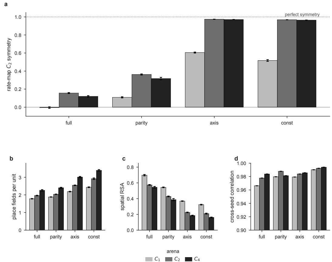
Figure 10. Quantifying the fold. (a) Rate-map C_2 symmetry index (correlation of a unit's map with its 180° rotation). It saturates near 0.97 when the encoding is invariant and the arena is symmetric, up to the perfect-symmetry line at 1; but note the C_1 baseline, where an invariant encoding alone drives it to 0.61 though nothing can fold, so this is a descriptive readout, not a fold-specific one. (b) Mean place fields per unit; rises with both arena symmetry and encoding invariance, but also in the C_1 arena where nothing folds, so field count alone is confounded. (c) Spatial representational similarity falls as the encoding is ablated and as arena symmetry increases. Like field count, it is confounded: most of the fall is present in the C_1 arena, where nothing folds, so it evidences that the code stays spatial rather than that it folds. (d) Cross-seed correlation between independently trained networks stays above 0.96 throughout (y zoomed to 0.9–1.0): descriptive evidence that the fold is reproducible rather than degenerate. No null is reported for this measure and none is claimed. Arenas C_1/C_2/C_4 ; bars are mean \pm s.e.m. over networks ( n = 6 per encoding for C_1 and C_2 , n = 4 for C_4 ; 64 networks in all). The unit-level symmetry-index distributions reported in the text are computed per unit over the full 112-network sweep (56,000 units).
