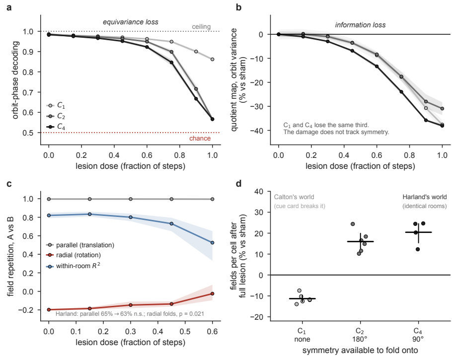
Figure 11. An in-silico head-direction lesion separates what the compass tells the map from what it does to it. Networks trained with an intact compass, which is then silenced at test time on a fraction of steps (zeroed, not randomised: an ablated head-direction system carries no signal, it does not carry a false one). n = 6 networks for C_1 and C_2 , n = 4 for C_4 ; shading, 95% bootstrap CI over networks. (a) Equivariance loss. Orbit-phase decoding (which of two symmetry-related places is the animal in?) collapses to chance in C_2 and C_4 and holds at 0.862 in C_1 , where no such pair exists ( t = 70.2 , p = 3 \times 10^{-19} ). (b) Information loss. Orbit variance (is the quotient map still there at all?) falls by about a third in every arena. The drops are not statistically identical ( F = 10.78 , p = 0.002 ) but they are not ordered by symmetry: C_1 (−37.6%) and C_4 (−38.1%) sit at opposite ends of the symmetry range and lose indistinguishable amounts, while C_2 (−30.9%) loses least. Panels (a) and (b) together are the argument: the same lesion degrades the quotient map without regard to symmetry and folds it only where a symmetry exists. (c) Harland's 2 \times 2 , in silico. The parallel arm is the reachable null: a compass is translation-invariant by construction, so it was never holding those rooms apart, and it does not move ( 0.996 \rightarrow 0.996 ). The radial arm rises. Within-room R^2 (blue) is the positive control: it must stay positive, or the repetition number is two destroyed maps correlating with each other. It does, up to dose 0.6, and we make no claim beyond that. (d) Field count after a full lesion, one dot per network: fields fall by 11% where nothing can fold and rise by 16% and 20% where something can, the same dissociation Harland and Calton et al. (2003) report in two different worlds.
