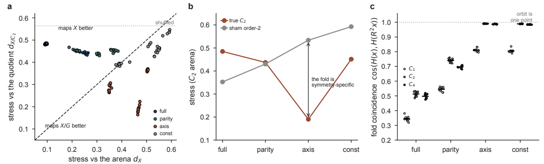
Figure 7. The folded manifold is a map of the quotient. One dot per network ( n = 10 per condition, 8 for C_4 ); stress is Kruskal stress-1 at optimal scale, lower is a better fit. (a) Fit to the arena metric d_X against fit to the quotient metric d_{X/C_2} , with the line of equal fit. full and parity lie above it, so they are better described as maps of X ; axis lies below it, so it is better described as a map of X/C_2 . Dotted line, the stress returned when the code's spatial content is destroyed by shuffling, a reachable ceiling. (b) The control for the compression artefact: d_{X/G} \leq d_X pointwise, so any group shrinks long distances. A sham order-2 group (translation by half the arena) compresses identically but is not a symmetry, and the folded code prefers the true C_2 over it by 0.343. (c) The same claim without any metric: the cosine between the population state at x and at its 180^\circ image. Under axis in the C_2 arena it is 0.990, so the orbit is one point; under parity , which carries the same one bit, it is 0.741.
