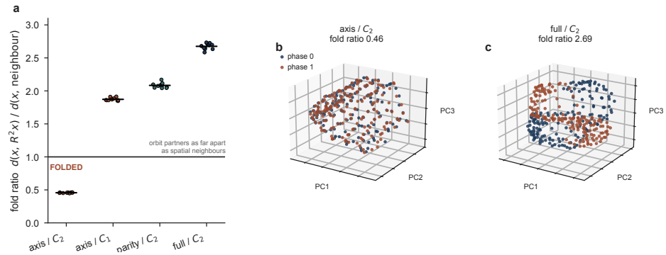
Figure 6. The fold, seen geometrically. (a) The fold ratio: the distance between a cell's population state and that of its 180^\circ image, in units of the distance to an adjacent cell. One dot per network, n = 10 per condition; bar, mean; whiskers, 95% bootstrap interval. Below one, orbit partners sit closer together than spatial neighbours do, which is what folding means. Only axis in the C_2 arena is below one ( 0.457 \pm 0.004 ); the same encoding with no symmetry to fold onto is not ( axis / C_1 , 1.872), nor is parity / C_2 (2.083), nor full / C_2 (2.675). The ratio is computed in the full hidden space, so it is not an artefact of the projection used to plot it: the folded case reads below one and every non-folded case above one under nonlinear embeddings (Isomap, t-SNE) as well as PCA. (b, c) Position-conditioned population manifold of the most- and the least-folded condition (one point per arena cell, PCA to three dimensions, coloured by C_2 orbit phase), illustrative; the fold ratio in (a) is the quantitative claim. The two phases superimpose under axis / C_2 and occupy separate regions under full / C_2 . We reduce with PCA because the claim is metric, that two positions coincide, and unlike neighbour-graph embeddings PCA preserves distances rather than reshaping them.
