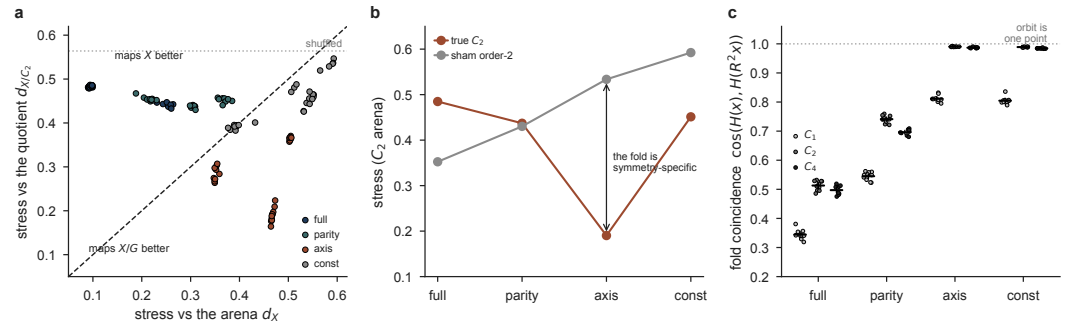
Figure 6. The folded manifold is a map of the quotient. One dot per network ( n = 10 per condition, 8 for C_4 ); stress is Kruskal stress-1 at optimal scale, lower is a better fit. (a) Fit to the arena metric d_X against fit to the quotient metric d_{X/C_2} , with the line of equal fit. full and parity lie above it, so they are better described as maps of X ; axis lies below it, so it is better described as a map of X/C_2 . Dotted line, the stress returned when the code's spatial content is destroyed by shuffling, a reachable ceiling. (b) The control for the compression artefact: d_{X/G} \leq d_X pointwise, so any group shrinks long distances. A sham order-2 group (translation by half the arena) compresses identically but is not a symmetry, and the folded code prefers the true C_2 over it by 0.343. (c) The same claim without any metric: the cosine between the population state at x and at its 180^\circ image. Under axis in the C_2 arena it is 0.990, so the orbit is one point; under parity , which carries the same one bit, it is 0.741.
