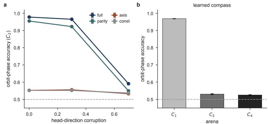
Figure 9. The quotient survives a degraded and a learned compass. (a) HD-lesion dose-response: orbit-phase accuracy in the C_2 arena as a function of the fraction of heading steps randomised (chance 0.5, dashed). The non-invariant encodings ( full , parity ) degrade smoothly, while the invariant ones ( axis , const ) stay pinned at chance. (b) A learned, angular-velocity compass, by arena: it resolves C_1 (0.97) but folds C_2 and C_4 to chance, building the quotient with no imposed encoding.
