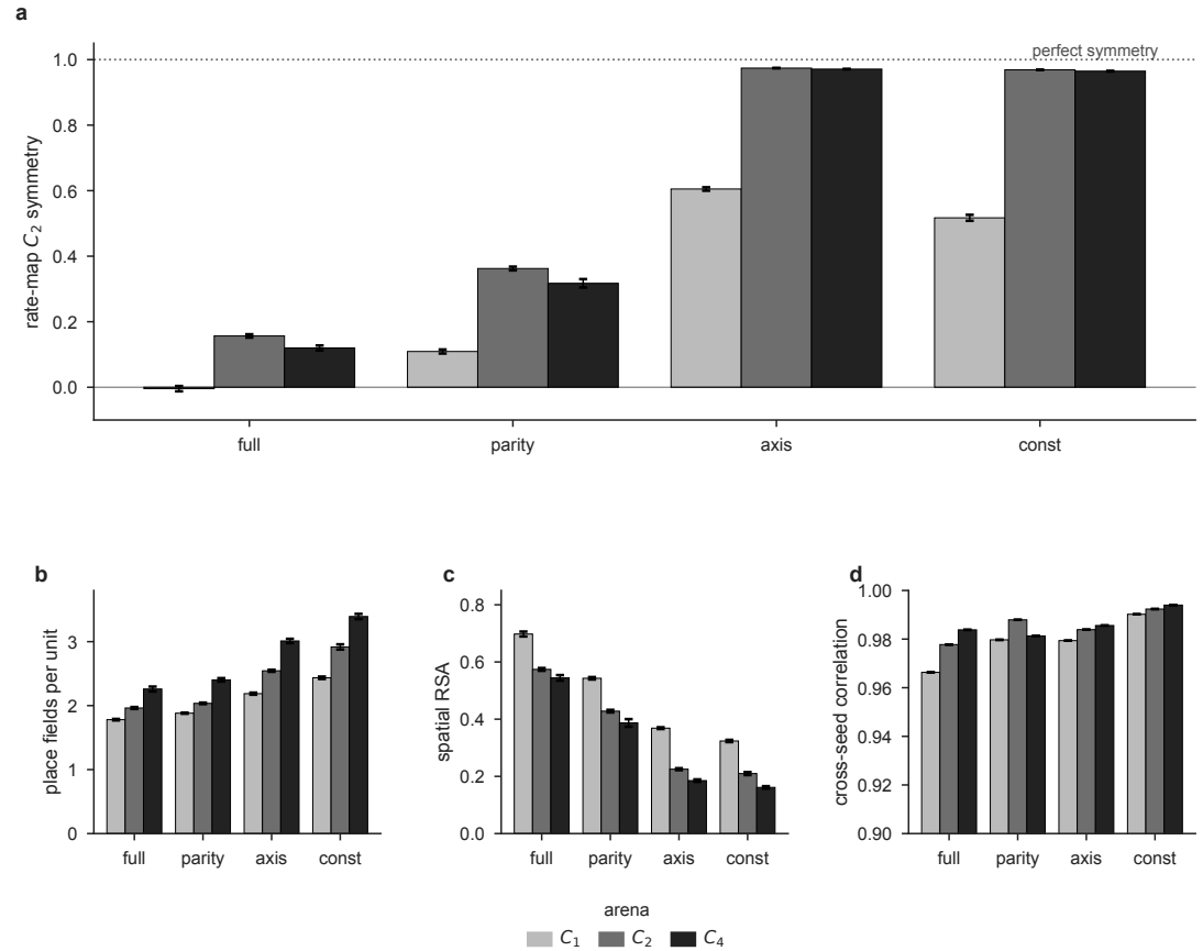
Figure 10. Quantifying the fold. (a) Rate-map C_2 symmetry index (correlation of a unit's map with its 180^\circ rotation), the fold-specific readout; it saturates near 0.97 only when the encoding is invariant to the arena's symmetry, up to the perfect-symmetry line at 1. (b) Mean place fields per unit; rises with both arena symmetry and encoding invariance, but also in the C_1 arena where nothing folds, so field count alone is confounded. (c) Spatial representational similarity falls as the encoding is ablated and as arena symmetry increases. Like field count, it is confounded: most of the fall is present in the C_1 arena, where nothing folds, so it evidences that the code stays spatial rather than that it folds. (d) Cross-seed correlation between independently trained networks stays above 0.96 throughout (y zoomed to 0.9–1.0): the fold is reproducible, not degenerate. Arenas C_1/C_2/C_4 ; bars are mean \pm s.e.m. over networks ( n = 10 per encoding for C_1 and C_2 , n = 8 for C_4 ).
