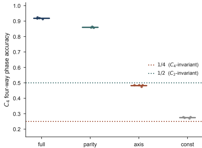
Figure 7. The C_4 arena reproduces the group-theoretic ceiling. Four-way orbit-phase accuracy in the C_4 arena (one dot per network; bar, mean; chance 0.25). A code folded onto X/G can name the coset but not the orbit element, so a |G| -way decoder is bounded by 1/|G| . const , invariant under the full C_4 group, falls to the 1/4 ceiling (dotted); the C_2 -invariant axis falls to the 1/2 ceiling; full and parity , not invariant, stay high. Ceilings are the group-theoretic predictions, not fits.
