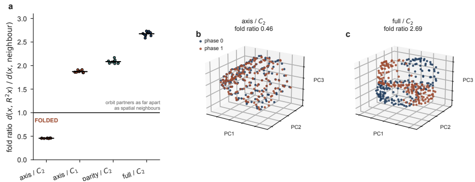
Figure 5. The fold, seen geometrically. (a) The fold ratio: the distance between a cell's population state and that of its 180^\circ image, in units of the distance to an adjacent cell. One dot per network, n = 10 per condition; bar, mean; whiskers, 95% bootstrap interval. Below one, orbit partners sit closer together than spatial neighbours do, which is what folding means. Only axis in the C_2 arena is below one ( 0.457 \pm 0.004 ); the same encoding with no symmetry to fold onto is not ( axis / C_1 , 1.872), nor is parity / C_2 (2.083), nor full / C_2 (2.675). The ratio is computed in the full hidden space, so it is not an artefact of the projection used to plot it: the folded case reads below one and every non-folded case above one under distance-preserving nonlinear embeddings (Isomap, t-SNE) as well as PCA. (b, c) Position-conditioned population manifold of the most- and the least-folded condition (one point per arena cell, PCA to three dimensions, coloured by C_2 orbit phase), illustrative; the fold ratio in (a) is the quantitative claim. The two phases superimpose under axis / C_2 and occupy separate regions under full / C_2 . We reduce with PCA because the claim is metric, that two positions coincide, and unlike neighbour-graph embeddings PCA preserves distances rather than reshaping them.
