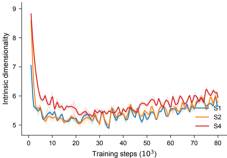
Manifold Dimensionality
