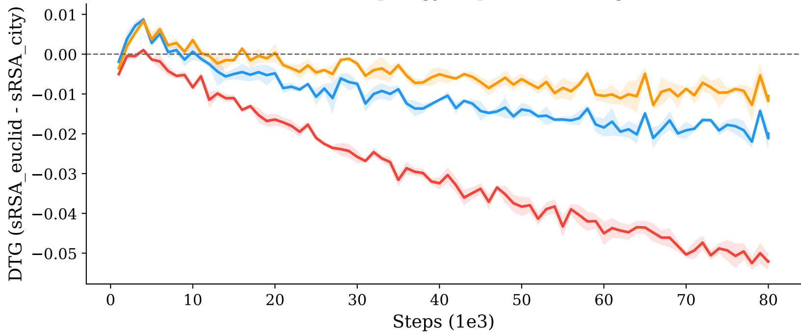
Distance-Topology Gap over training
