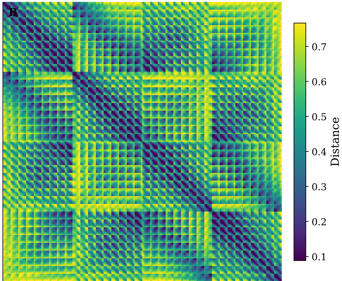
Observed neural RDM
