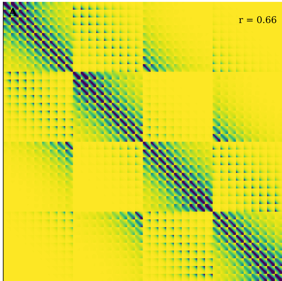
Predicted SR geometry (rescaled)
