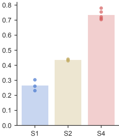
Spectral Gap
