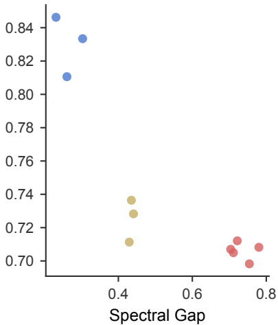
sRSA
