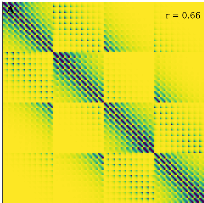
Predicted SR geometry (rescaled)
