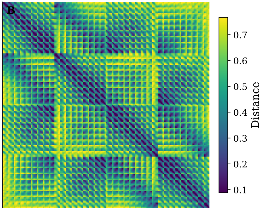
Observed neural RDM
