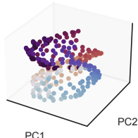
theta ( b_1 = 2 ) 35% var
