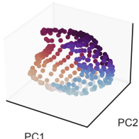
open ( b_1 = 0 ) 41% var
