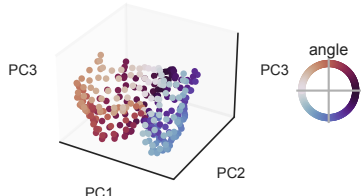
figure-8 ( b_1 = 2 ) 34% var
