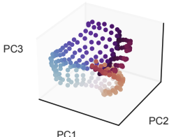
annulus ( b_1 = 1 ) 34% var
