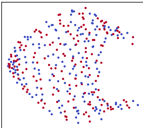
s2/parity fold=2.72
