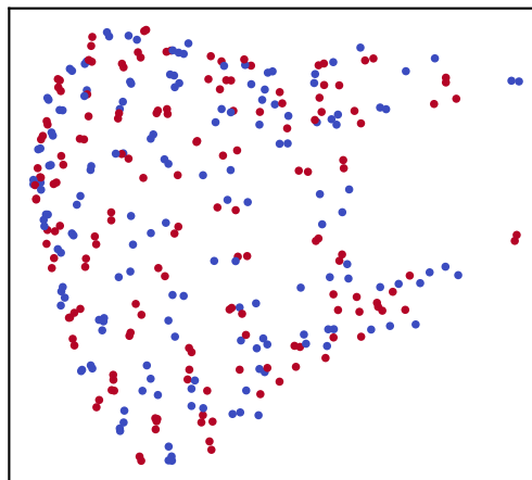
s2/axis fold=0.22
