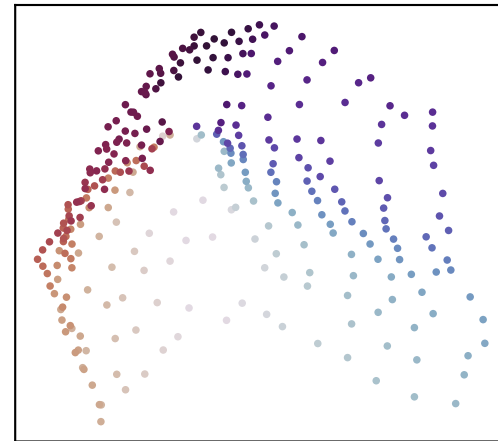
figure8 loop=0.79
