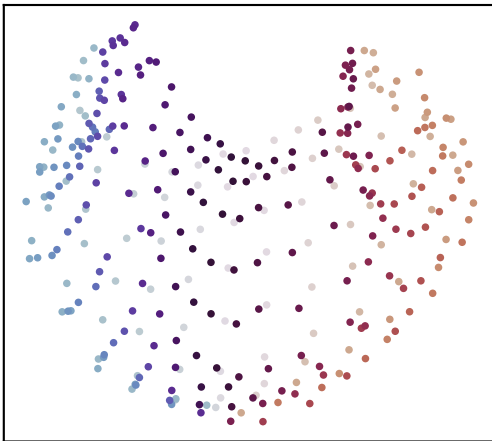
s2/full fold=3.79
