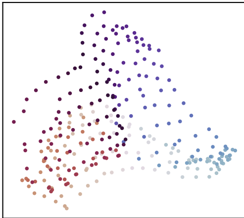
s2/parity fold=2.72
