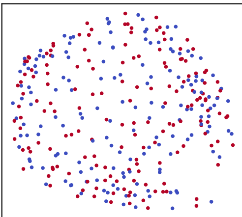
s2/full fold=3.79
