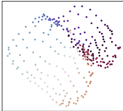
s2/axis fold=0.22
