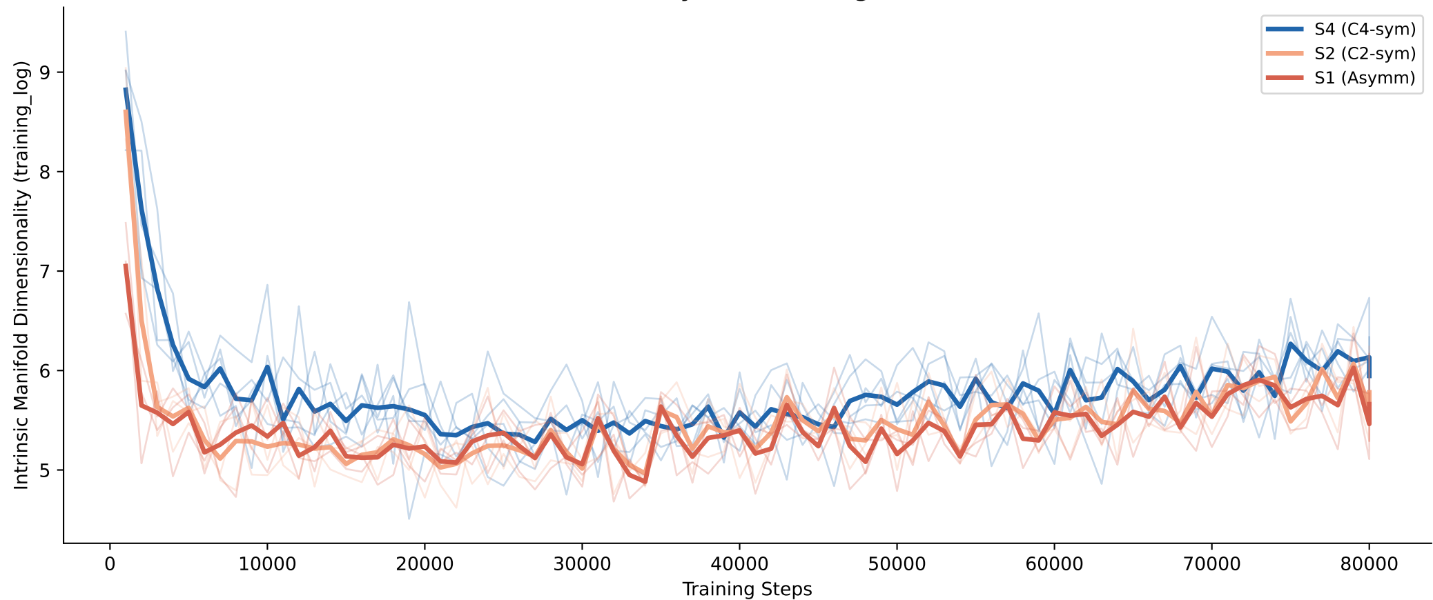
Manifold Dimensionality Over Training (online estimator)
