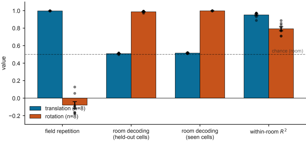
Place-field repetition across identical compartments
