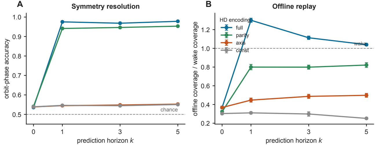
Figure 4. Symmetry resolution and offline replay across the prediction horizon k , in the C_2 arena, for the four head-direction encodings. Left: orbit-phase decoding accuracy (chance 0.5). The two encodings that are not C_2 -invariant ( full , parity ) resolve the fold at k \geq 1 , while the two invariant ones ( axis , const ) stay at chance. Right: coverage of the self-generated offline trajectory as a fraction of a wake path of equal length; the dashed line marks wake coverage. Both readouts step up at k = 1 and are ordered by how much of the compass the encoding retains. Points are mean \pm s.e.m. over n = 6 networks.
