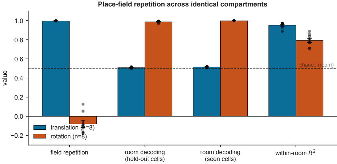
Figure 7. Place-field repetition across two observationally identical compartments. Under translation (parallel rooms) fields repeat and the room is undecodable, at chance even for a decoder tested on cells it has seen. Under rotation (radial rooms) fields do not repeat and the room is fully decodable. Within-room position ( R^2 ) is high in both, so neither network has stopped coding space. Bars are mean \pm s.e.m.; dots are individual networks.
