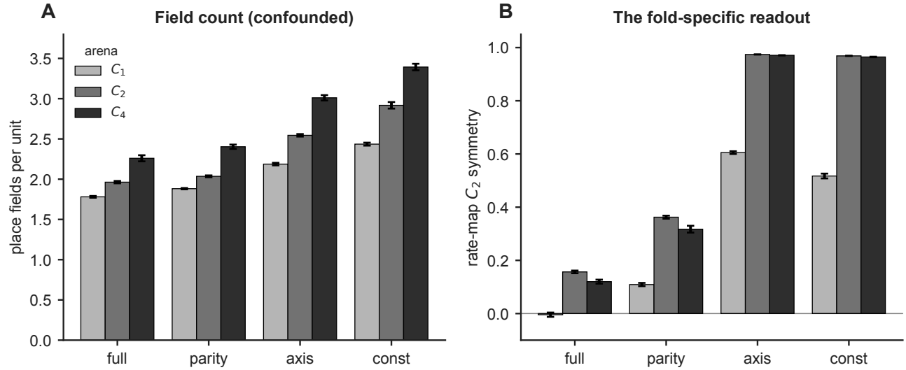
Figure 6. Place-field structure across arenas and encodings. (A) Mean number of place fields per unit. It increases with both arena symmetry and encoding invariance, but also in the C_1 arena where nothing folds, so it is confounded. (B) The rate-map C_2 symmetry index, the correlation of a unit's map with its 180^\circ rotation. This fold-specific measure saturates near 0.97 only when the encoding is invariant to the arena's symmetry, and stays low for the non-invariant encodings. Bars are mean \pm s.e.m. over networks.
