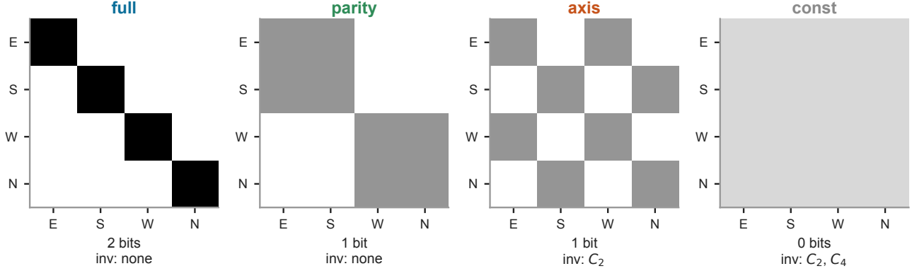
Figure 1. The four head-direction encodings, as 4 \times 4 transforms of the one-hot heading block {E, S, W, N}. full is the identity (two bits); parity and axis each collapse the compass to one bit but partition the headings differently; const discards it entirely. axis and const are invariant under the 180^\circ rotation and so fold the C_2 arena, while const is the only encoding invariant under the full C_4 group. axis and parity carry identical information and differ only in this invariance.
