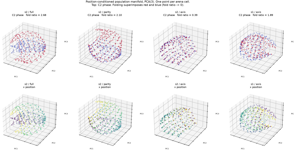
Figure 3. Position-conditioned population manifold (one point per arena cell, PCA to three dimensions), coloured by C_2 orbit phase. Under full and parity the two phases occupy separate regions; under axis in the C_2 arena they superimpose. The fold ratio — distance between a cell and its 180^\circ image, in units of the distance to a spatial neighbour — is 2.68, 2.10 and 0.39 respectively, and 1.89 for axis in the C_1 arena, where the same encoding folds nothing.
