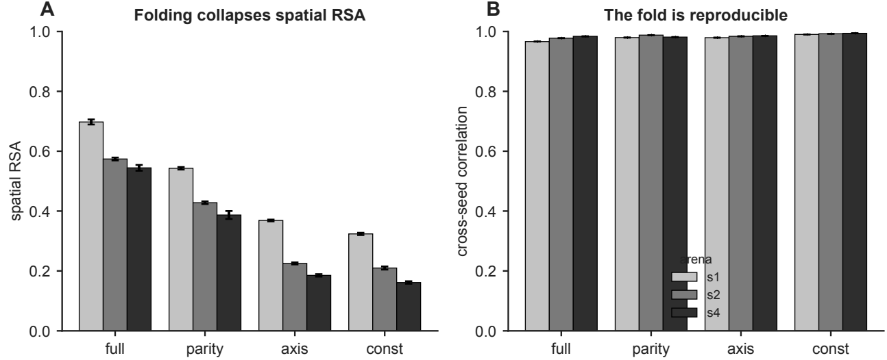
Figure 5. A map forms and folds reproducibly. Left: spatial representational similarity falls as the head-direction encoding is ablated ( full to const ) and as arena symmetry increases ( C_1 to C_4 ), the signature of a code collapsing onto the quotient. Right: the cross-seed correlation between independently trained networks stays above 0.96 throughout, so the folding is consistent rather than degenerate. Bars are mean \pm s.e.m. over networks.
