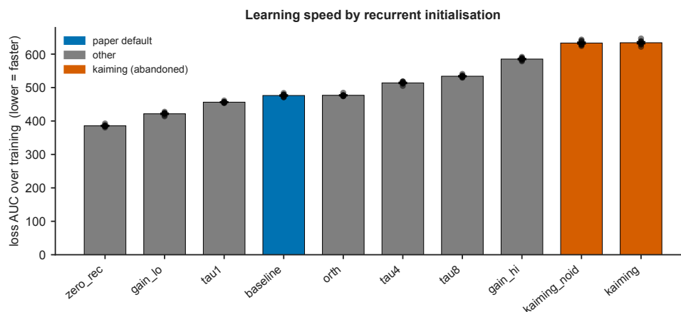
Figure S9. Learning speed by recurrent initialization, measured as area under the training-loss curve (lower is faster), ranked. A pure leak with no random recurrence learns fastest; adding random mixing slows learning monotonically. The abandoned Kaiming initialization is slowest but converges without instability. Dots are individual networks.
