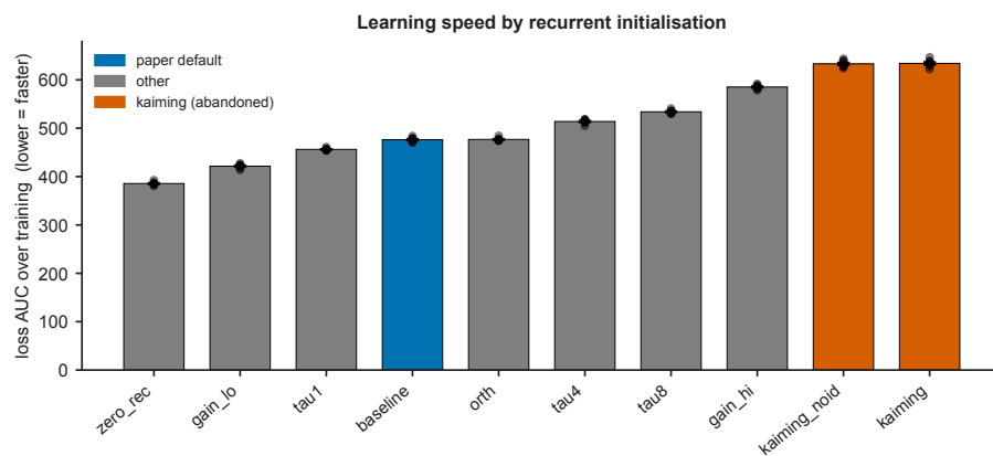
Figure S8. Learning speed by recurrent initialisation, measured as area under the training-loss curve (lower is faster). A pure leak learns fastest; the abandoned Kaiming initialisation is slowest but converges without instability.
