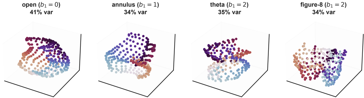
Figure S5. Position-conditioned population manifolds for the four topology arenas, PCA to three dimensions (one point per passable cell, coloured by angle around the arena centre). Position is mapped smoothly in every arena, but the manifolds are high-dimensional: three principal components capture only 34–41% of the variance, and no low-dimensional loop is visible even for the annulus ( b_1 = 1 ) or the theta and figure-8 arenas ( b_1 = 2 ). This is consistent with the persistent-homology analysis, which does not recover the arenas' loop topology (main text, Limitations): the code is metrically organised well before, and without ever cleanly acquiring, the arena's topology.
