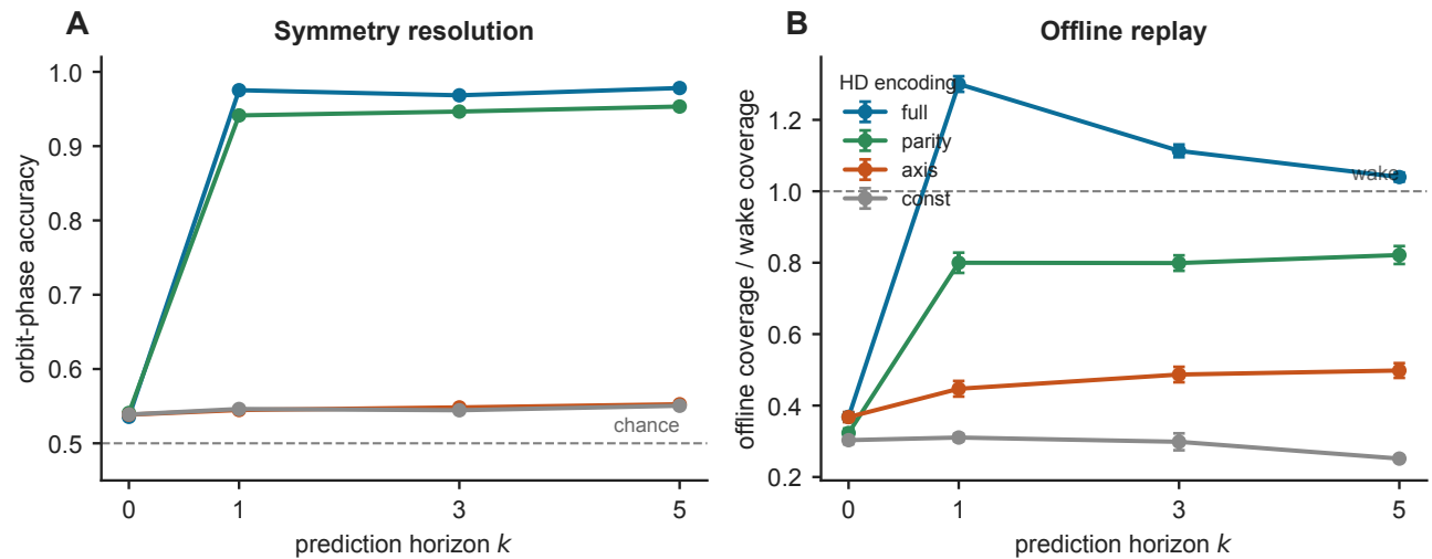
Figure S7. Symmetry resolution (left) and offline replay coverage (right) as a function of the prediction horizon k , for the four head-direction encodings in the C_2 arena. Both step up at k = 1 and are graded by how much of the compass the encoding retains.
