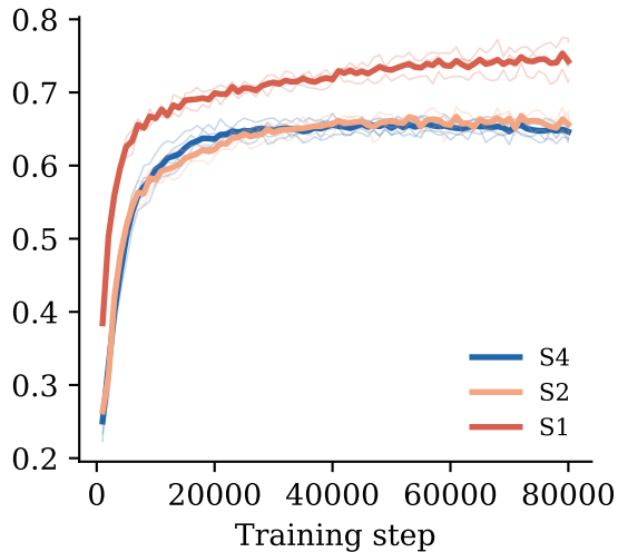
spatial_sRSA
