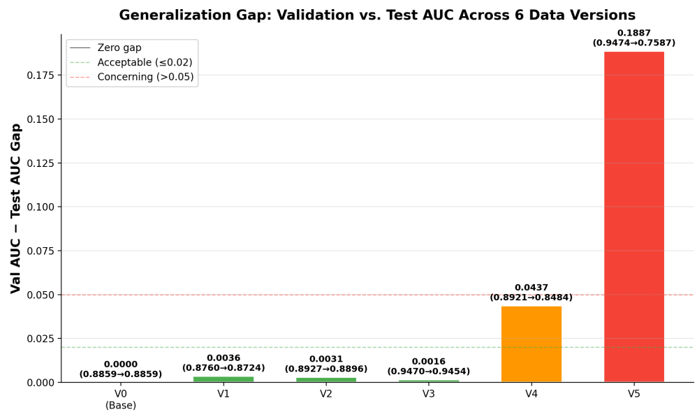
Figure 5.20: Generalization gap (Val AUC minus Test AUC) across all six data versions. Green bars indicate minimal overfitting (gap \leq 0.02 ), orange bars indicate moderate overfitting (0.02–0.05), and red bars indicate severe overfitting (gap > 0.05 ).
