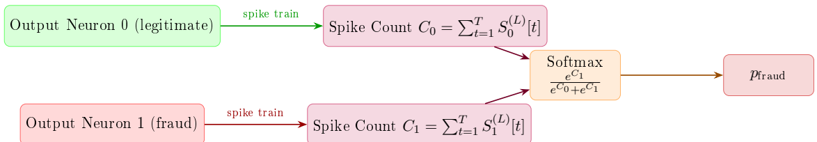
Figure 6.2: Spike count decoding and probability extraction. The output spike trains from the two output neurons are aggregated over T time steps, and the softmax function converts the spike counts into a fraud probability estimate.
