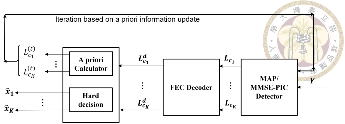
Figure 4.3: The block diagram of the MAP-IDD/MMSE-PIC-IDD receiver
