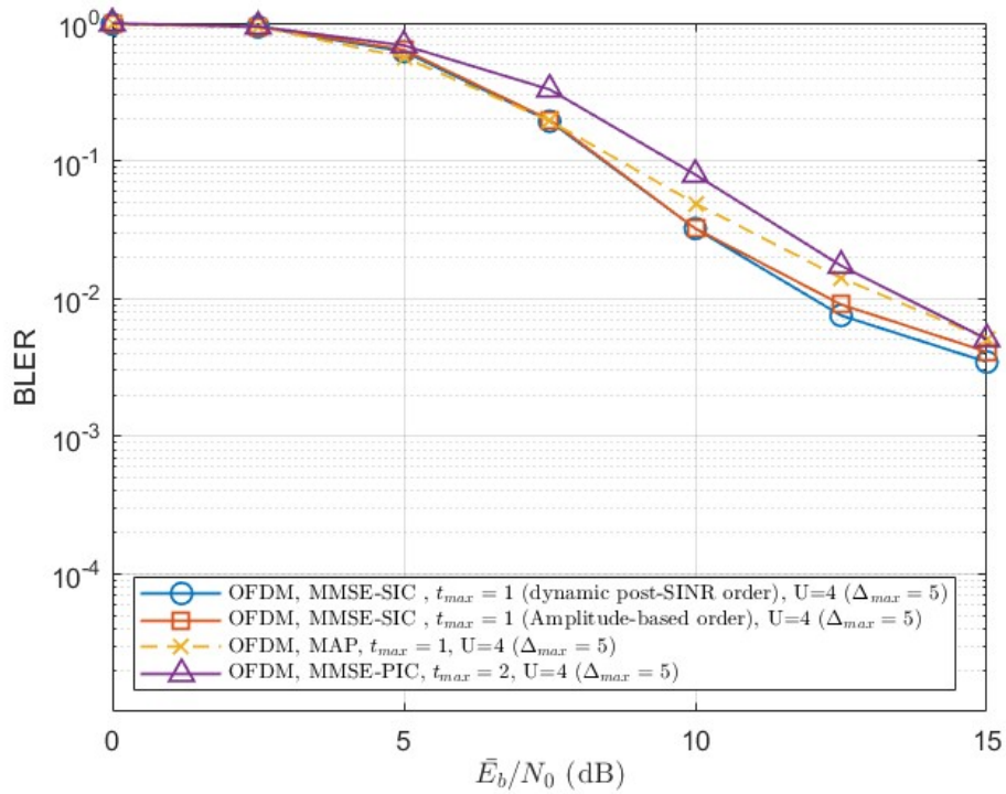
Figure 4.23: BLER of asynchronous OFDM system with MMSE-SIC-IDD, MMSE-PIC-IDD, and MAP-IDD. R = 2 , U = 4 , \Delta_{\max} = 5 , t_{\max} = 1 for MMSE-SIC-IDD and MAP-IDD.
