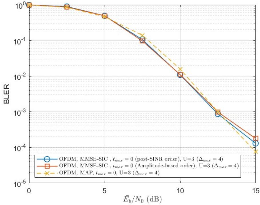
Figure 4.16: BLER of asynchronous OFDM system with MMSE-SIC-IDD and MAP-IDD. R = 2 , U = 3 , \Delta_{\max} = 4 , t_{\max} = 0 .
