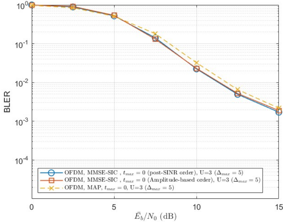
Figure 4.18: BLER of asynchronous OFDM system with MMSE-SIC-IDD and MAP-IDD. R = 2 , U = 3 , \Delta_{\max} = 5 , t_{\max} = 0 .
