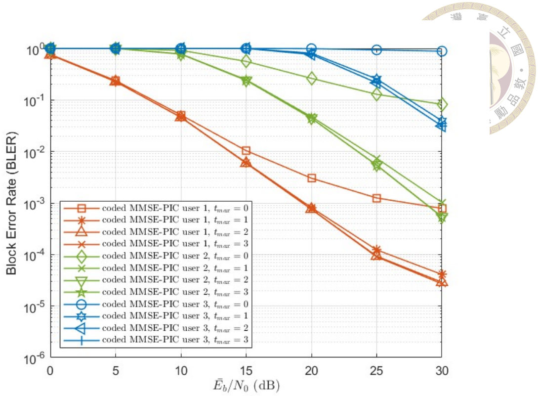
Figure 4.5: BLER of MMSE-PIC-IDD with R = 2 , (\beta_1, \beta_2, \beta_3) = (1, 0.1, 0.01) , t_{\max} = 0, 1, 2, 3
