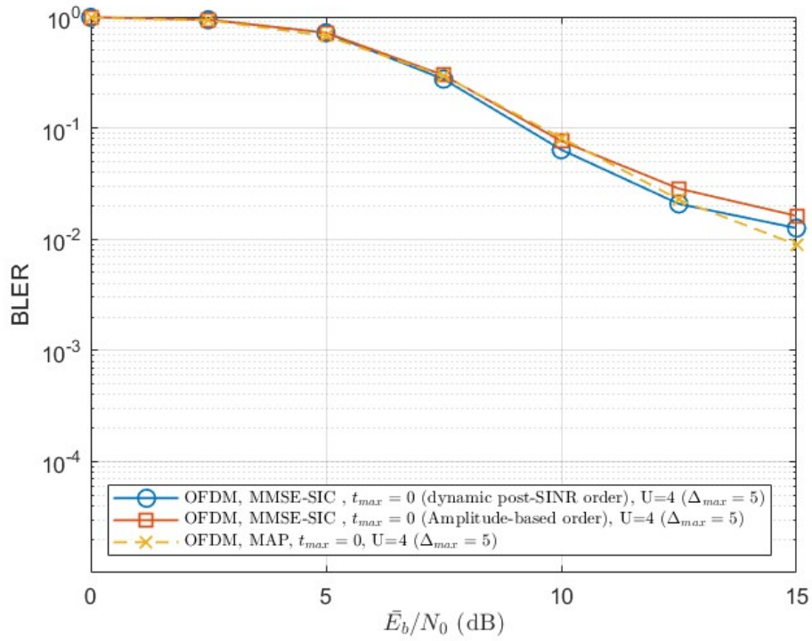
Figure 4.22: BLER of asynchronous OFDM system with MMSE-SIC-IDD and MAP-IDD. R = 2 , U = 4 , \Delta_{\max} = 5 , t_{\max} = 0 .
