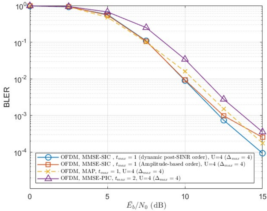
Figure 4.21: BLER of asynchronous OFDM system with MMSE-SIC-IDD, MMSE-PIC-IDD, and MAP-IDD. R = 2 , U = 4 , \Delta_{max} = 4 , t_{max} = 1 for MMSE-SIC-IDD and MAP-IDD.
