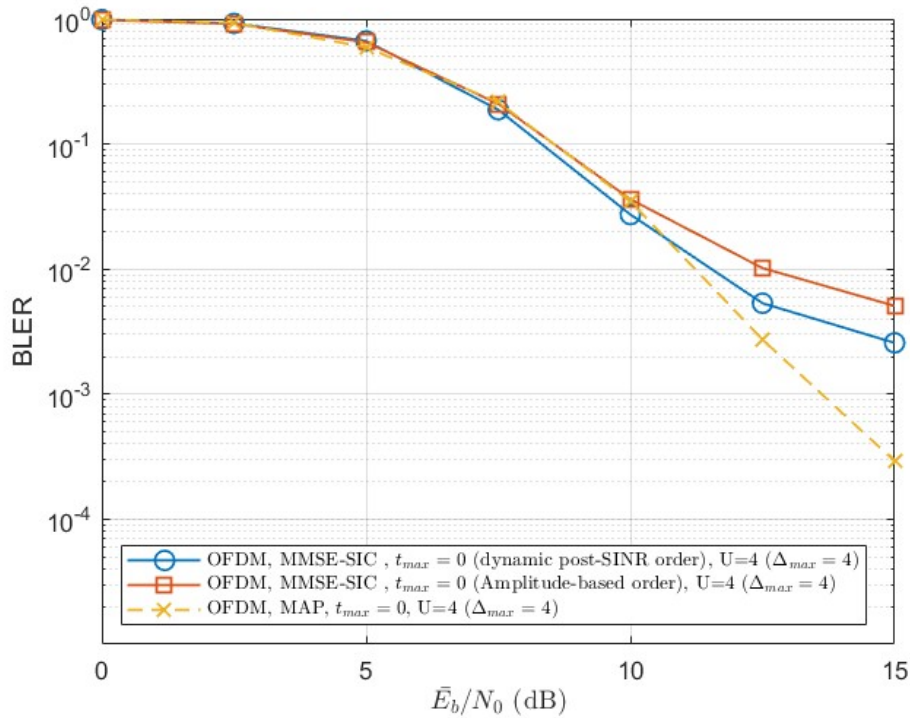
Figure 4.20: BLER of asynchronous OFDM system with MMSE-SIC-IDD and MAP-IDD. R = 2 , U = 4 , \Delta_{\max} = 4 , t_{\max} = 0 .
