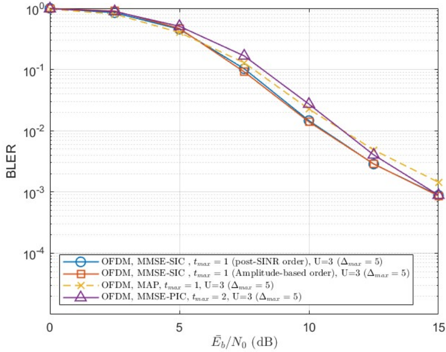
Figure 4.19: BLER of asynchronous OFDM system with MMSE-SIC-IDD, MMSE-PIC-IDD, and MAP-IDD. R = 2 , U = 3 , \Delta_{\max} = 5 , t_{\max} = 1 for MMSE-SIC-IDD and MAP-IDD.
