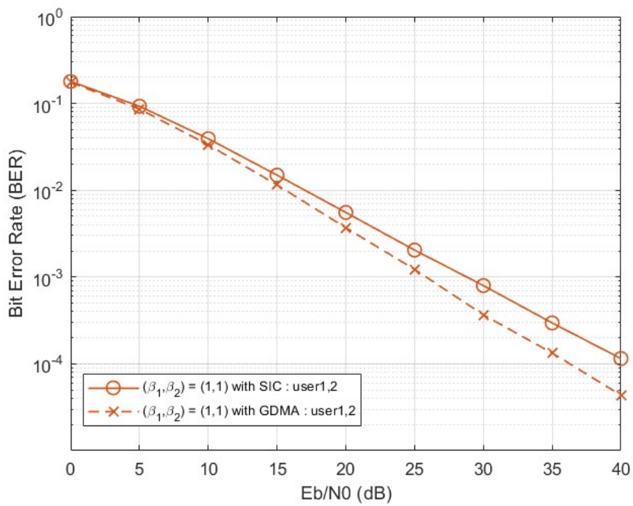
Figure 2.1: Users' BERs for single resource systems of (\beta_1, \beta_2) = (1, 1) .
