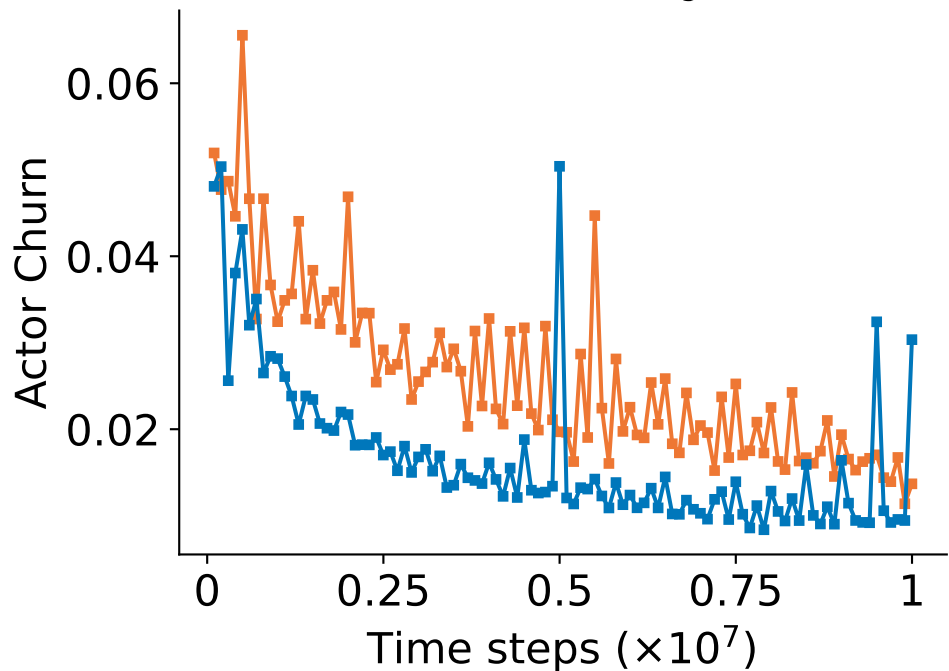
Actor Churn (KL divergence)
