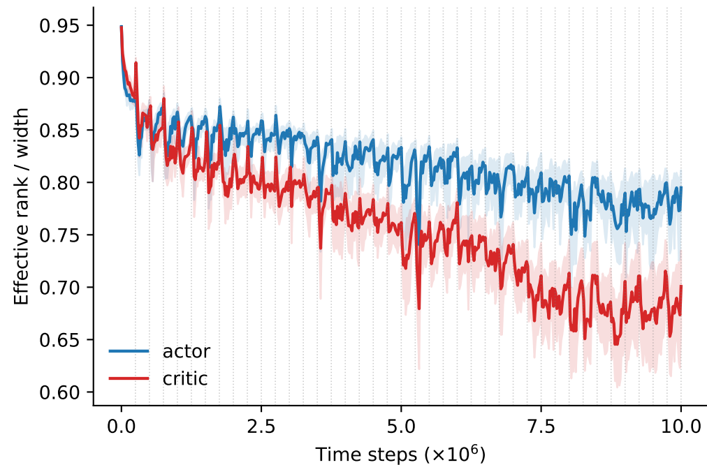
ReLU 1
