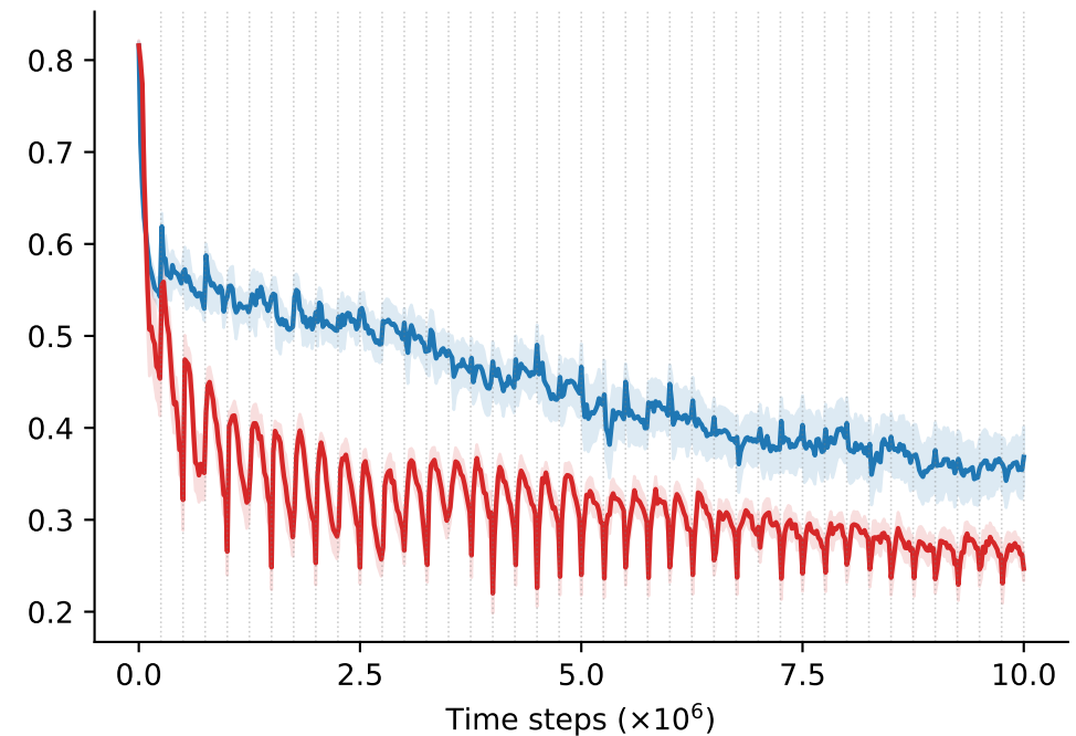
ReLU 2
