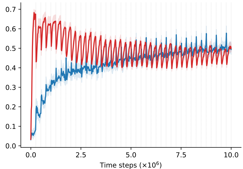
ReLU 2
