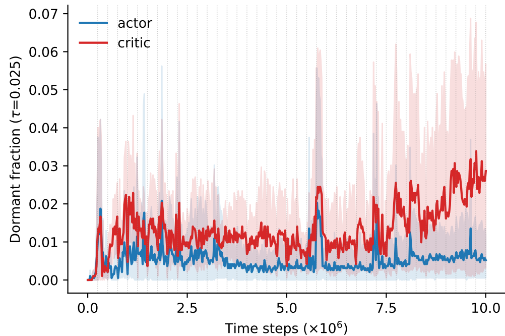
ReLU 1
