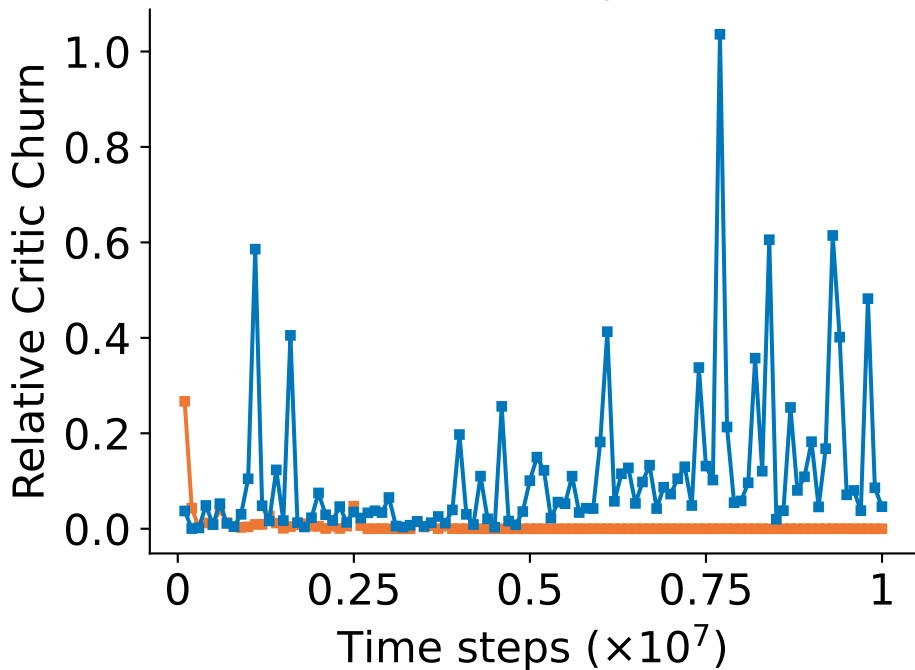
Critic Churn (magnitude)
