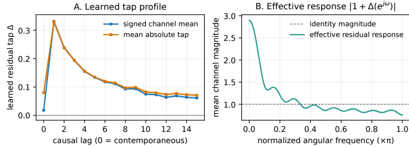
Fig. S1. Learned residual-tap and effective frequency-response summaries from the eight released selected checkpoints of the outcome-known active-control learned arm. Channels are summarized within each seed; bands are ordinary 95% t intervals over the eight seed summaries. Lag 0 is contemporaneous. These are descriptive fitted-operator diagnostics, not a mechanism or independent-confirmation test; plotted values are released in figures/fig_fir_response_data.csv . The effective kernel is the residual identity plus the learned \Delta taps.
