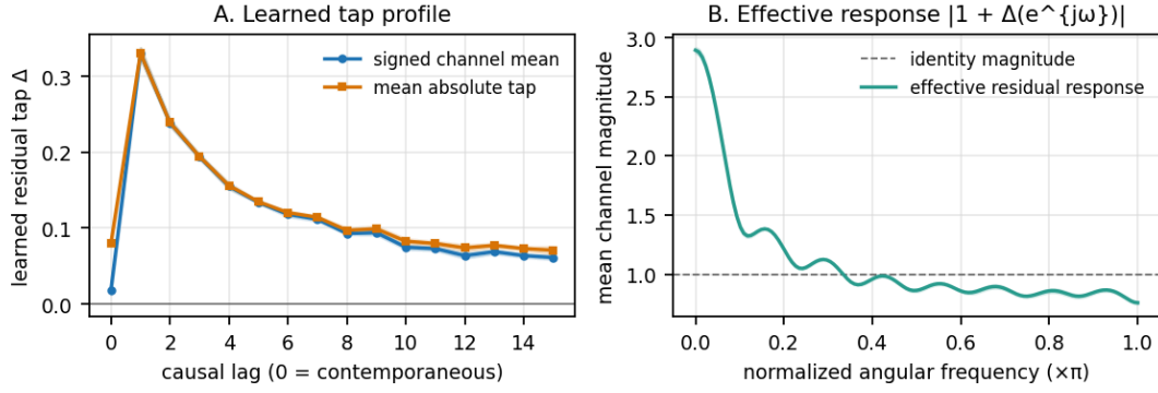
Fig. S1: Selected-checkpoint FIR diagnostics. The effective kernel is the residual identity plus the learned \Delta taps. The plot establishes neither temporal specificity nor learned-tap superiority; those require the active non-temporal placebo and prospective study described in §6.
