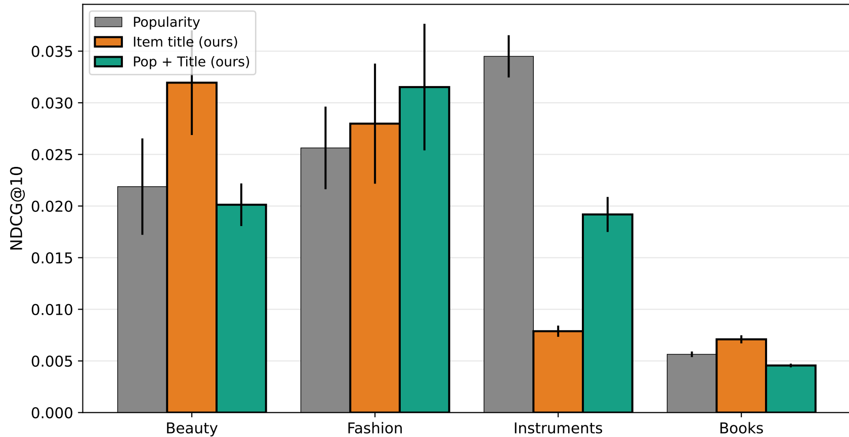
Cold-Start NDCG@10 (GroupKFold, few-shot context)
