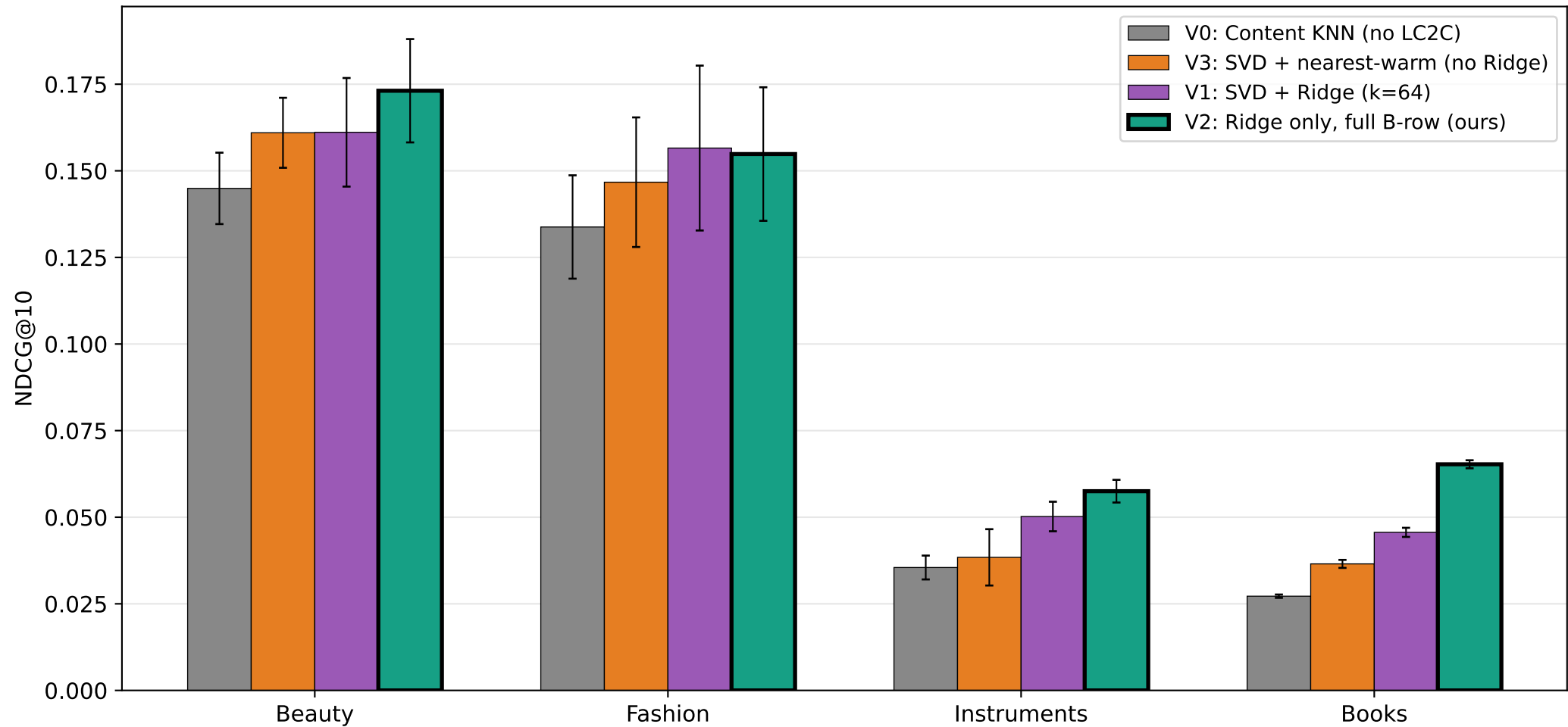
LC2C Component Ablation — does each piece contribute?
