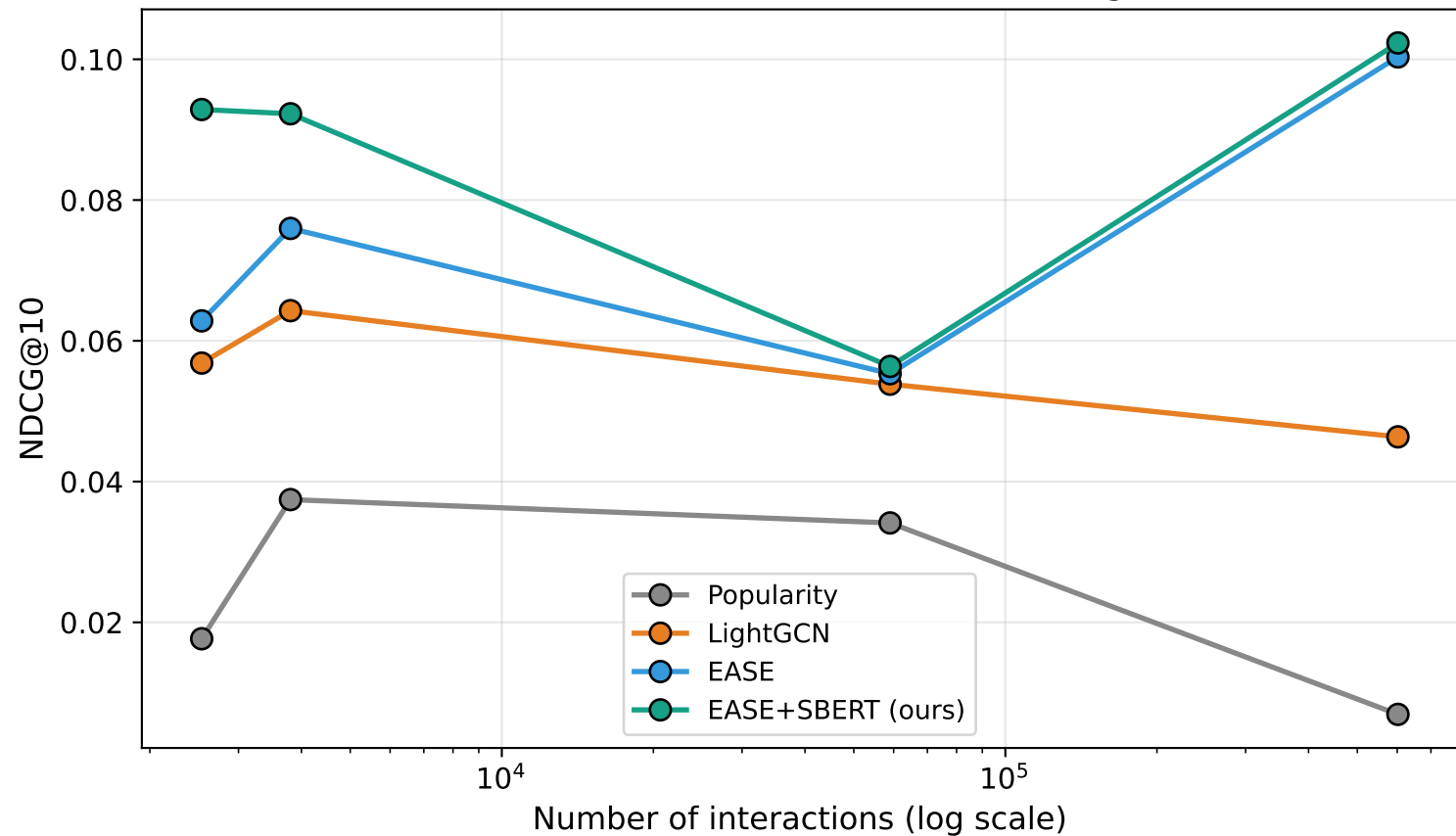
Method NDCG@10 vs Dataset Size (log)
