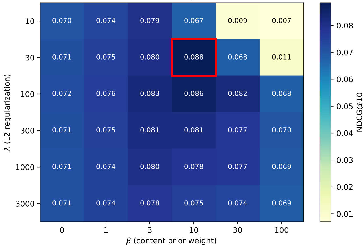
NDCG@10 sensitivity — Fashion
