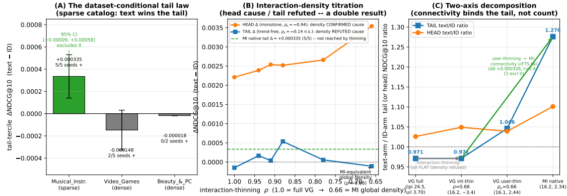
Dataset-conditional long-tail law and its two-axis causal decomposition (AR2023 5-core LLOO, full-catalog, NDCG@10; all values 5-seed best-by-val except Beauty 2-3 seed)
