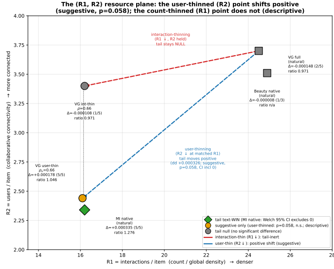
AR2023 5-core LLOO, full-catalog NDCG@10; VG runs 5-seed best-by-val ( n_{\text{eval}}=84,762 , tail n=10,900 frozen), Beauty 2-3 seed. The two VG thinned points share R1 = 16.2 (matched count) but differ in R2 ; only the R2 -thinned point moves to a positive tail point estimate beside MI (suggestive).
