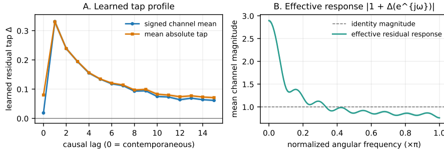
Fig. S1. Learned residual-tap and effective frequency-response summaries from the eight released selected checkpoints of the outcome-known active-control learned arm. Channels are summarized within each seed; bands are ordinary 95% t intervals over the eight seed summaries. Lag 0 is contemporaneous. These are descriptive fitted-operator diagnostics, not a mechanism or independent-confirmation test; plotted values are released in figures/fig_fir_response_data.csv . The effective kernel is the residual identity plus the learned \Delta taps.
