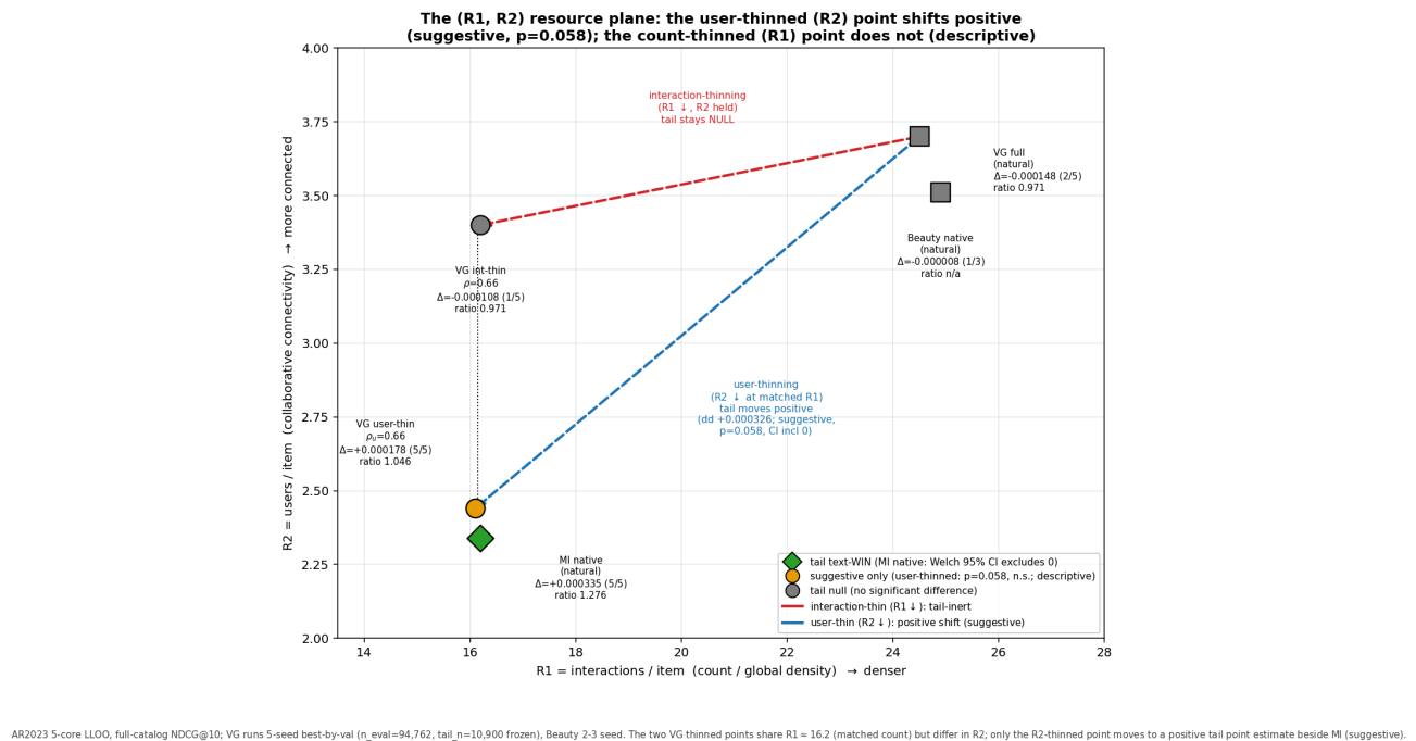
Fig. 2: The ( R1 = \text{interactions/item} , R2 = \text{users/item} ) resource plane — the two VG thinned rungs share R1 , but only the user-thinned ( R2 ) point moves to a positive tail point estimate beside MI native (suggestive; p = 0.058 ).
