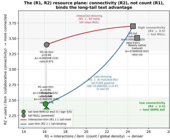
AR2023 5-core LLOO, full-catalog NDCG@10; VG runs 5-seed best-by-val ( n_{\text{eval}}=94,762 , n_{\text{tail}}=10,900 frozen), Beauty 2-3 seed. The two VG thinned points share R1 \approx 16.2 (matched count) but differ in R2; only the R2-thinned point crosses to a tail win, beside MI.
