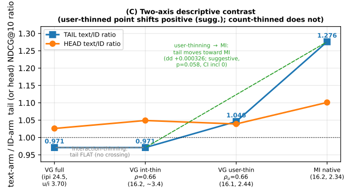
Fig. 3. (A) TFFV2 repaired-estimand tail contrasts — MI, VG, and the MI-VG interaction as Welch 95% CIs (8 fresh seeds per arm; one estimand; outcome-visible campaign, §5.3; cross-dataset heterogeneity not established, p = 0.13 ). The historical defective-cohort Table 1d values are tabulated, not plotted. (B) Interaction-density titration level contrasts and (C) two-axis descriptive ratios — both on ONE fixed subset draw with no draw/seed uncertainty shown; arms are not initialization-paired (§5.3); the panel-C shift is suggestive only ( p = 0.058 , CI includes 0). Plotted values, estimator, and analysis IDs: figures/fig_tail_law_mechanism_data.csv.
