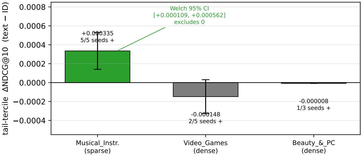
(A) The dataset-conditional tail pattern (sparse catalog: text wins the tail; TFV2: freq-5-heavy)
