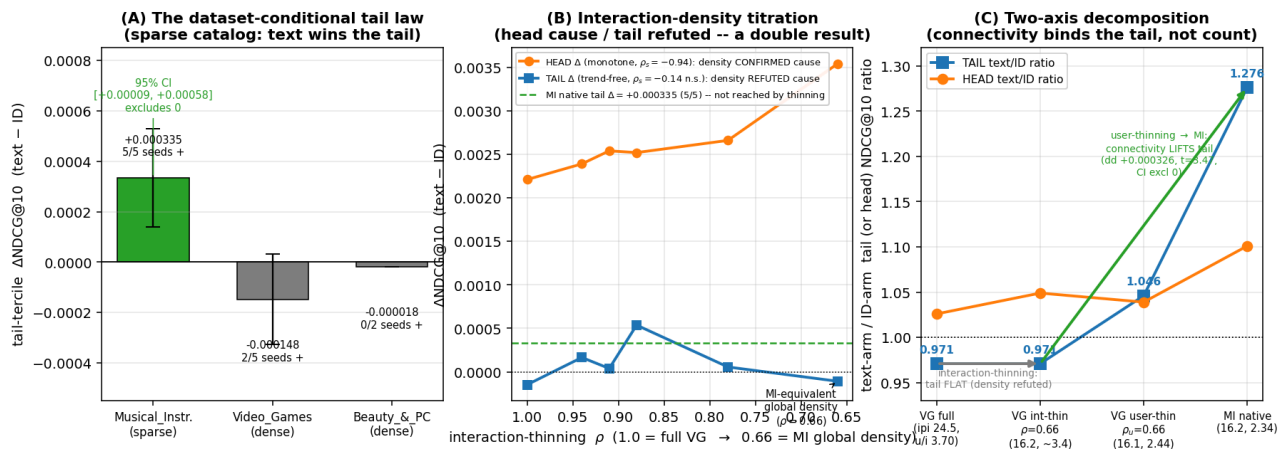
Fig. 1: The dataset-conditional tail pattern — per-seed paired text-ID tail deltas by category (Musical_Instruments win; Video_Games and Beauty powered nulls).
