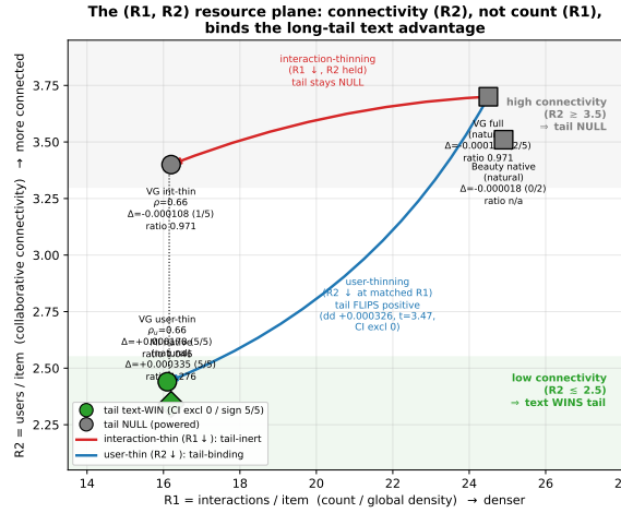
AR2023 5-core LLOO, full-catalog NDCG@10; VG runs 5-seed best-by-val ( n_{\text{eval}}=94,762 , tail, n=10,900 frozen), Beauty 2-3 seed. The two VG thinned points share R1 \approx 16.2 (matched count) but differ in R2; only the R2-thinned point crosses to a tail win, beside MI.
