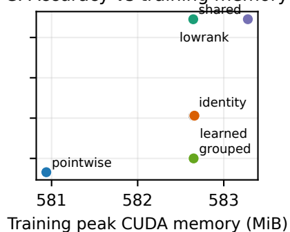
C. Accuracy vs training memory
