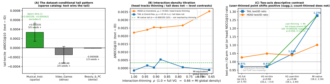
Fig. 1. The dataset-conditional tail pattern — same-seed-number text-ID tail deltas by category (Musical_Instruments win; Video_Games null, equivalence not established; Beauty exploratory). Panels: (A) the tail pattern; (B) the interaction-density titration level contrasts; (C) the connectivity-vs-count descriptive contrast. All panels summarize bundled interventions on one fixed subset draw — subset (draw) uncertainty is not represented, and the arms are not initialization-paired (§5.3 randomization disclosure).
