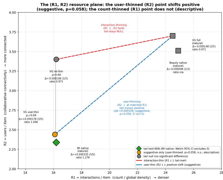
Fig. 2: The ( R_1 = interactions/item, R_2 = users/item) resource plane — the two VG thinned rungs share R_1 , but only the user-thinned ( R_2 ) point moves to a positive tail point estimate beside MI native (suggestive; p = 0.058 ).
