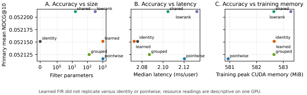
Fig. 2. MovieLens 1M R4 aggregate FIR accuracy-resource plane. Learned FIR failed to replicate versus identity and pointwise. Resource readings are descriptive on one GPU; exact aggregate values are in figures/fig_fir_efficiency_ml1m_v1_data.csv.
