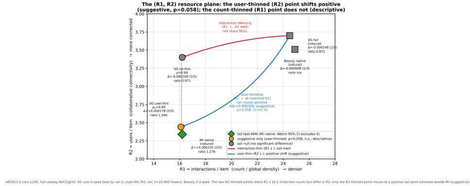
Fig. 2. The ( R1 = \text{interactions/item} , R2 = \text{users/item} ) resource plane — the two VG thinned rungs share R1 , but only the user-thinned ( R2 ) point moves to a positive tail point estimate beside MI native (suggestive, p = 0.058 ; descriptive contrast; bundled interventions on one fixed subset draw; the §5.4.2 dd inference is suggestive, not significant, under the corrected independent-arm analysis).
