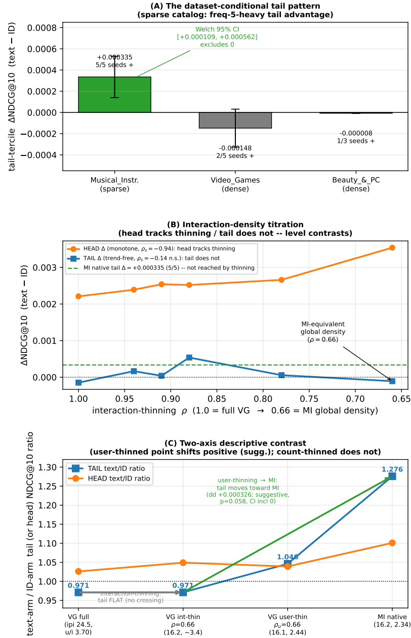
Fig. 1. The dataset-conditional tail pattern — same-seed-number text-ID tail deltas by category (Musical_Instruments win — frequency-5-heavy under TFFV2; Video_Games null, equivalence not established; Beauty exploratory). Panels: (A) the tail pattern; (B) the interaction-density titration level contrasts; (C) the connectivity-vs-count descriptive contrast. All panels summarize bundled interventions on one fixed subset draw — subset (draw) uncertainty is not represented, and the arms are not initialization-paired (9.3 randomization disclosure).
