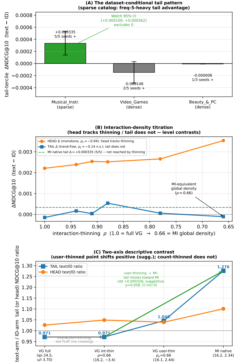
Fig. 1. The dataset-conditional tail pattern — same-seed-number text-ID tail deltas by category (Musical_Instruments win — frequency-5-heavy under TFV2; Video_Games null, equivalence not established; Beauty exploratory). Panels: (A) the tail pattern; (B) the interaction-density titration level contrasts; (C) the connectivity-vs-count descriptive contrast. All panels summarize bundled interventions on one fixed subset draw — subset (draw) uncertainty is not represented, and the arms are not initialization-paired (9.5 randomization disclosure).
