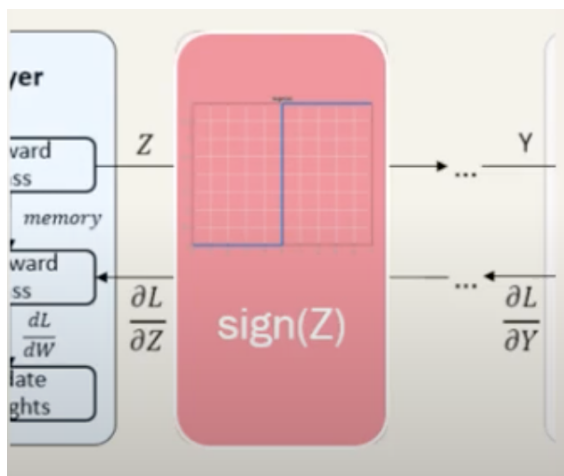
Figure 12.11: Zoomed-in look at one layer of BNN during training, showing use of STE during backpropagation.
